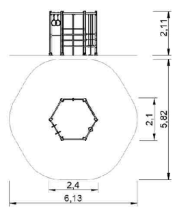
Estructura Hexagonal para Gimnasia Hexagonal Shaped Monkey Bars Structure à Agrès Hexagonale
