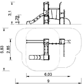
Multijuego Veleta Seis Torres Six Towers Veleta Playset Structure Multi-Jeux Veleta Six Tours
